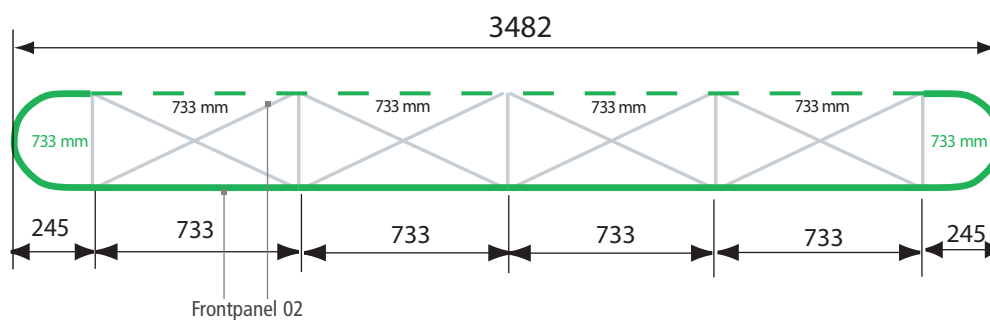
Pop Up Magnetic gerade, 4 x 3 Felder
