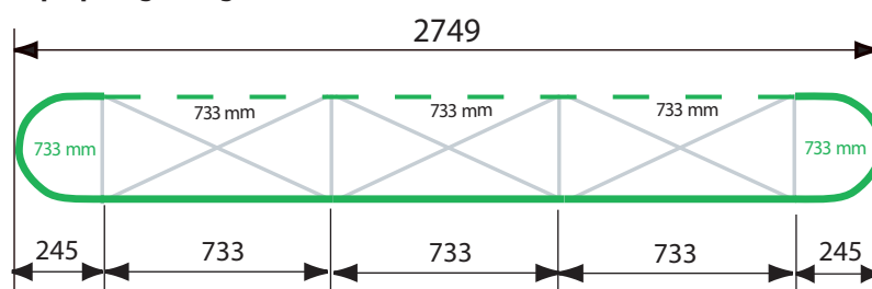
Pop Up Magnetic gerade, 3 x 3 Felder
